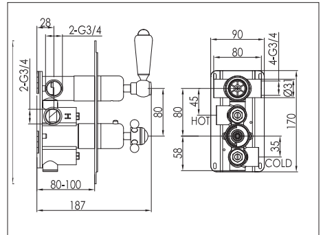
two-outlet
